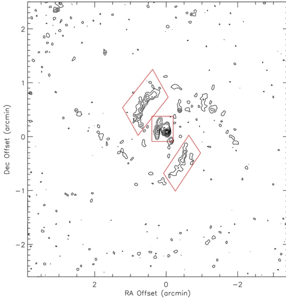
Figure 1. from Characterizing Magnetized Turbulence in M51 Houde et al. 2013 ApJ 766 49 doi:10.1088/0004-637X/766/1/49 https://dx.doi.org/10.1088/0004-637X/766/1/49 © 2013. The American Astronomical Society. All rights reserved.
