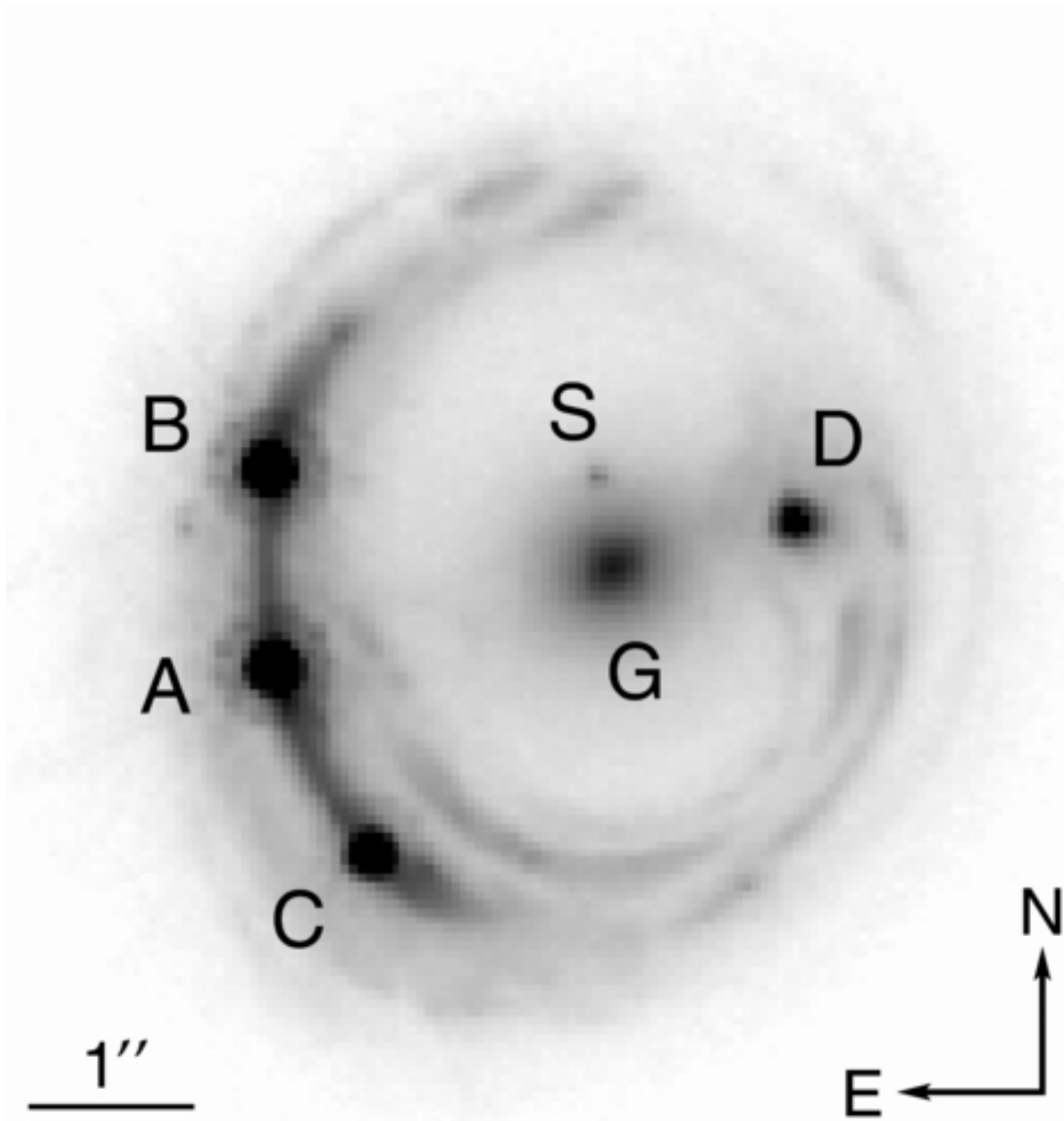
Figure 1. from Two Accurate Time-delay Distances from Strong Lensing: Implications for Cosmology Suyu et al. 2013 ApJ 766 70 doi:10.1088/0004-637X/766/2/70 https://dx.doi.org/10.1088/0004-637X/766/2/70 © 2013. The American Astronomical Society. All rights reserved.
