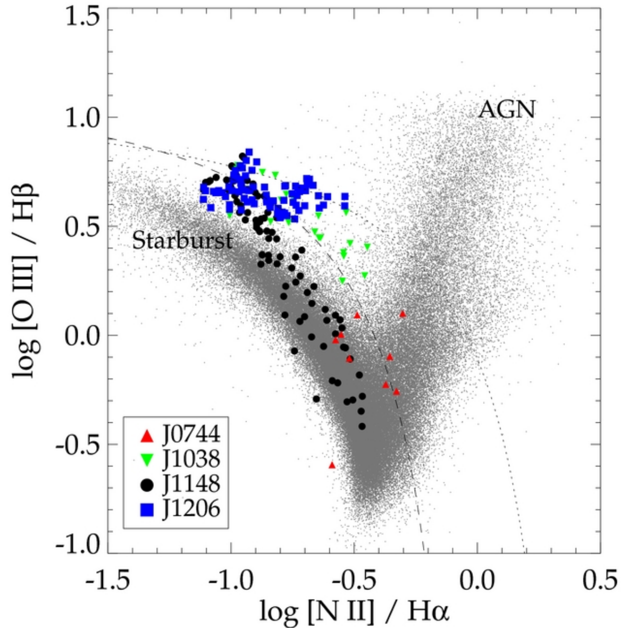
Figure 4. from The Origin and Evolution of Metallicity Gradients: Probing the Mode of Mass Assembly at z \sim 2 Jones et al. 2013 ApJ 765 48 doi:10.1088/0004-637X/765/1/48 https://dx.doi.org/10.1088/0004-637X/765/1/48 © 2013. The American Astronomical Society. All rights reserved.
