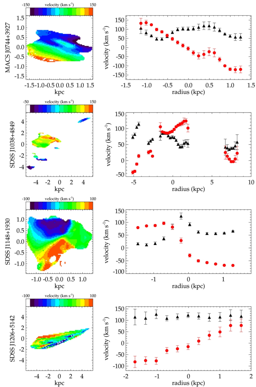
Figure 3. from The Origin and Evolution of Metallicity Gradients: Probing the Mode of Mass Assembly at z \sim 2 Jones et al. 2013 ApJ 765 48 doi:10.1088/0004-637X/765/1/48 https://dx.doi.org/10.1088/0004-637X/765/1/48
