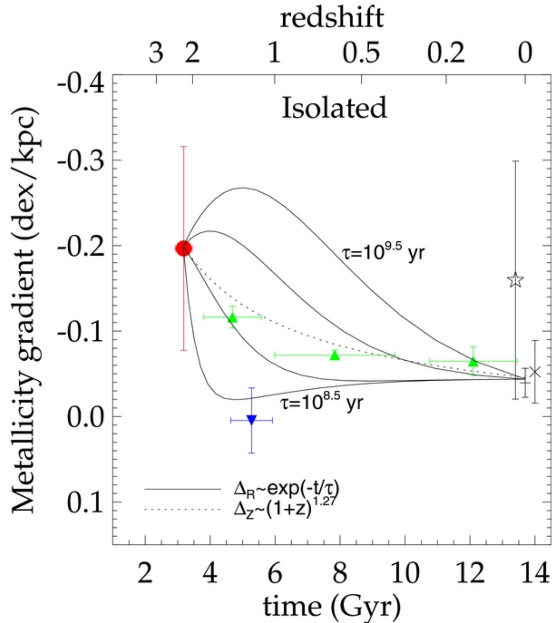
Figure 10. from The Origin and Evolution of Metallicity Gradients: Probing the Mode of Mass Assembly at z \gtrsim 2 Jones et al. 2013 ApJ 765 48 doi:10.1088/0004-637X/765/1/48 https://dx.doi.org/10.1088/0004-637X/765/1/48 © 2013. The American Astronomical Society. All rights reserved.
