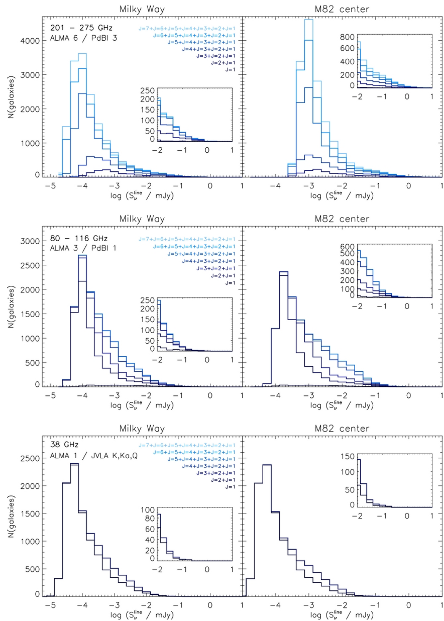
Figure 9. from Empirical Predictions for (Sub-)millimeter Line and Continuum Deep Fields da Cunha et al. 2013 ApJ 765 9 doi:10.1088/0004-637X/765/1/9 https://dx.doi.org/10.1088/0004-637X/765/1/9
