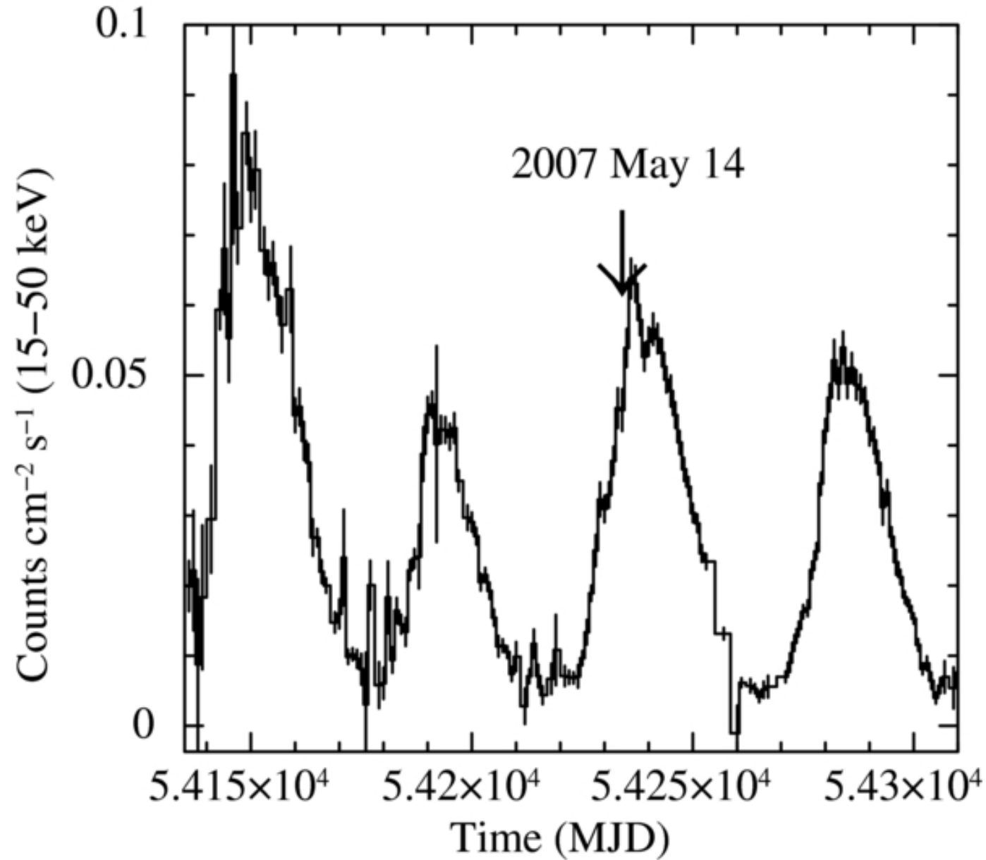
Figure 1. from Timing and Spectral Properties of Be/X-Ray Pulsar EXO 2030+375 during a Type I Outburst Naik et al. 2013 ApJ 764 158 doi:10.1088/0004-637X/764/2/158 https://dx.doi.org/10.1088/0004-637X/764/2/158 © 2013. The American Astronomical Society. All rights reserved.
