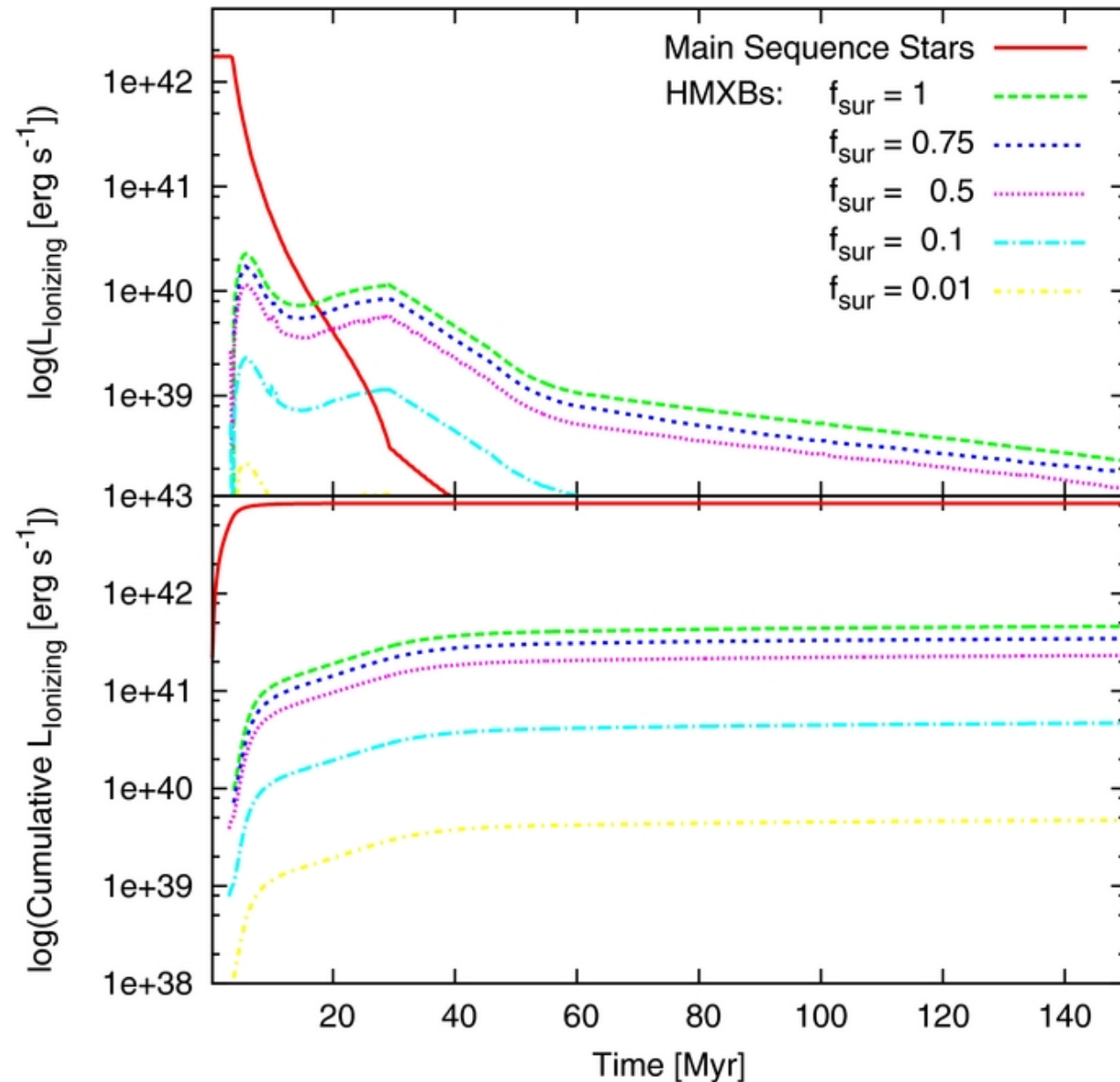
Figure 2. from Feedback from High-mass X-Ray Binaries on the High-redshift Intergalactic Medium: Model Spectra Power et al. 2013 ApJ 764 76 doi:10.1088/0004-637X/764/1/76 https://dx.doi.org/10.1088/0004-637X/764/1/76 © 2013. The American Astronomical Society. All rights reserved.
