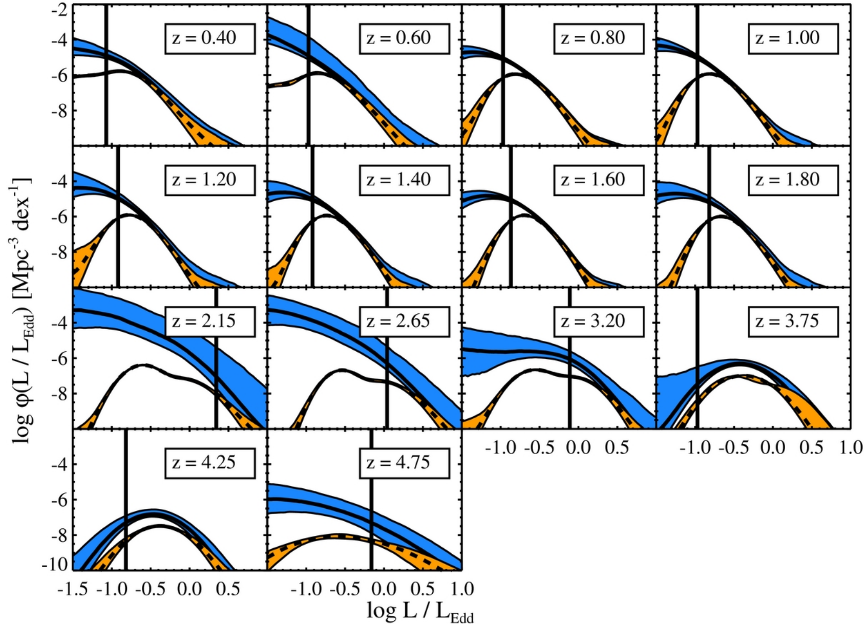
Figure 9. from The Demographics of Broad-line Quasars in the Mass-Luminosity Plane. II. Black Hole Mass and Eddington Ratio Functions Kelly & Shen 2013 ApJ 764 45 doi:10.1088/0004-637X/764/1/45 https://dx.doi.org/10.1088/0004-637X/764/1/45 © 2013. The American Astronomical Society. All rights reserved.
