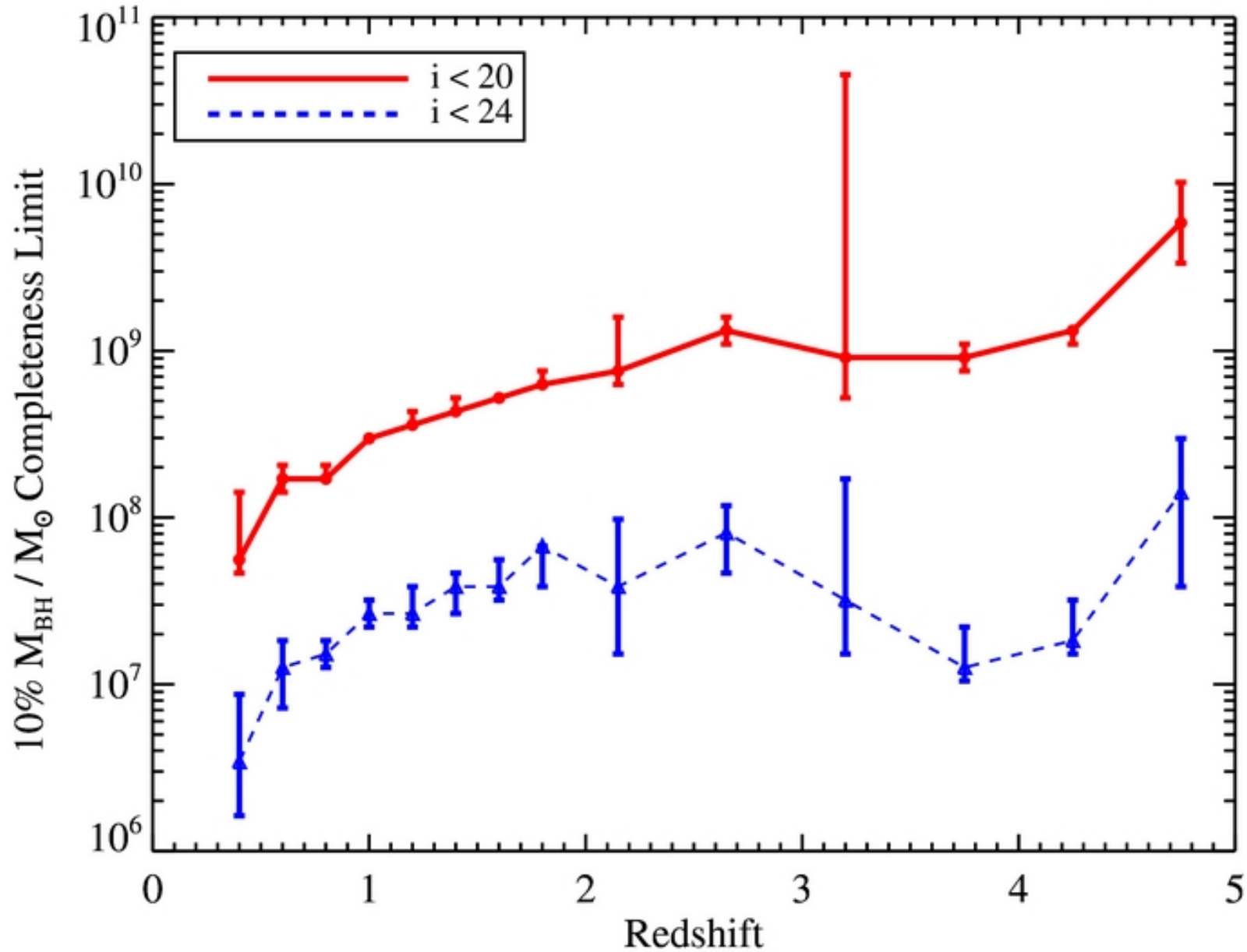
Figure 8. from The Demographics of Broad-line Quasars in the Mass-Luminosity Plane. II. Black Hole Mass and Eddington Ratio Functions Kelly & Shen 2013 ApJ 764 45 doi:10.1088/0004-637X/764/1/45 https://dx.doi.org/10.1088/0004-637X/764/1/45 © 2013. The American Astronomical Society. All rights reserved.
