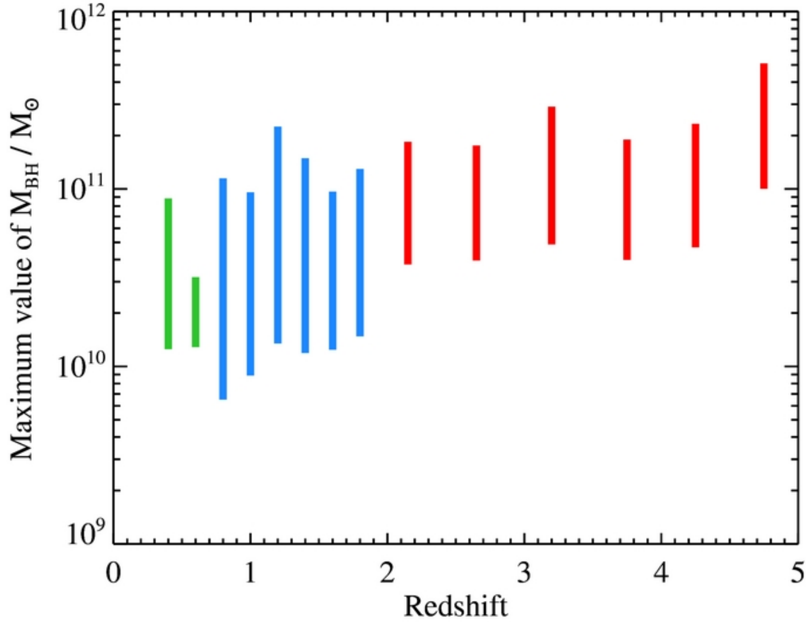
Figure 7. from The Demographics of Broad-line Quasars in the Mass-Luminosity Plane. II. Black Hole Mass and Eddington Ratio Functions Kelly & Shen 2013 ApJ 764 45 doi:10.1088/0004-637X/764/1/45 https://dx.doi.org/10.1088/0004-637X/764/1/45 © 2013. The American Astronomical Society. All rights reserved.
