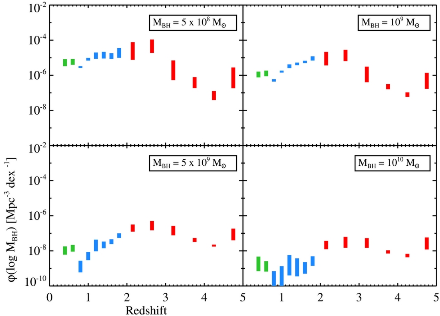
Figure 5. from The Demographics of Broad-line Quasars in the Mass-Luminosity Plane. II. Black Hole Mass and Eddington Ratio Functions Kelly & Shen 2013 ApJ 764 45 doi:10.1088/0004-637X/764/1/45 https://dx.doi.org/10.1088/0004-637X/764/1/45 © 2013. The American Astronomical Society. All rights reserved.
