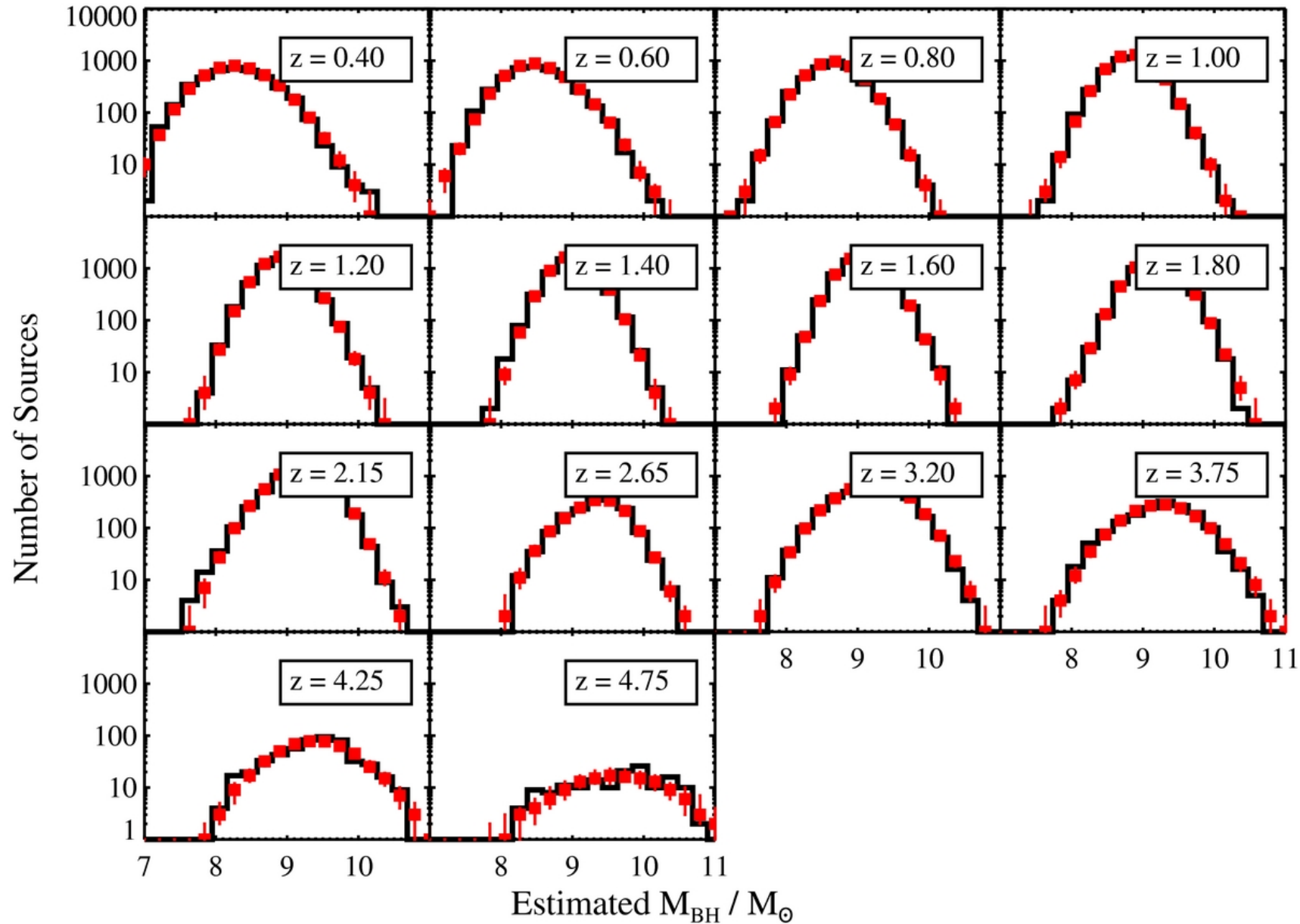
Figure 3. from The Demographics of Broad-line Quasars in the Mass-Luminosity Plane. II. Black Hole Mass and Eddington Ratio Functions Kelly & Shen 2013 ApJ 764 45 doi:10.1088/0004-637X/764/1/45 https://dx.doi.org/10.1088/0004-637X/764/1/45 © 2013. The American Astronomical Society. All rights reserved.
