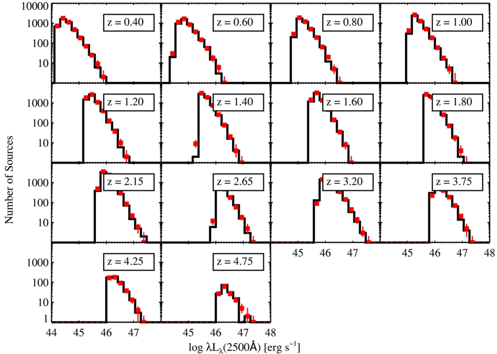
Figure 2. from The Demographics of Broad-line Quasars in the Mass-Luminosity Plane. II. Black Hole Mass and Eddington Ratio Functions Kelly & Shen 2013 ApJ 764 45 doi:10.1088/0004-637X/764/1/45 https://dx.doi.org/10.1088/0004-637X/764/1/45 © 2013. The American Astronomical Society. All rights reserved.
