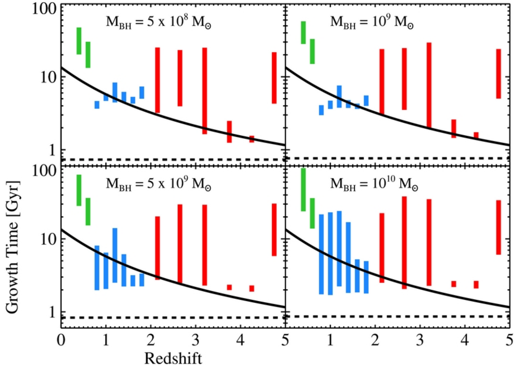
Figure 15. from The Demographics of Broad-line Quasars in the Mass-Luminosity Plane. II. Black Hole Mass and Eddington Ratio Functions Kelly & Shen 2013 ApJ 764 45 doi:10.1088/0004-637X/764/1/45 https://dx.doi.org/10.1088/0004-637X/764/1/45 © 2013. The American Astronomical Society. All rights reserved.
