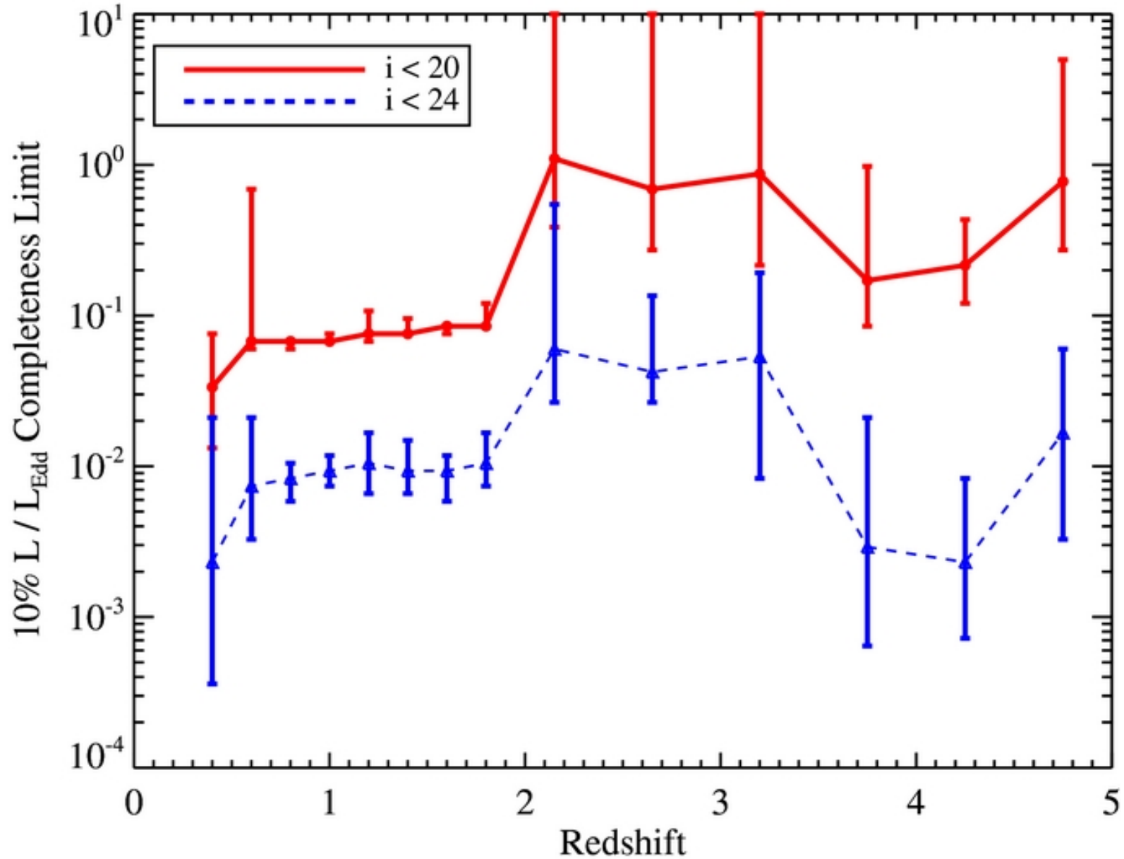
Figure 14. from The Demographics of Broad-line Quasars in the Mass-Luminosity Plane. II. Black Hole Mass and Eddington Ratio Functions Kelly & Shen 2013 ApJ 764 45 doi:10.1088/0004-637X/764/1/45 https://dx.doi.org/10.1088/0004-637X/764/1/45 © 2013. The American Astronomical Society. All rights reserved.
