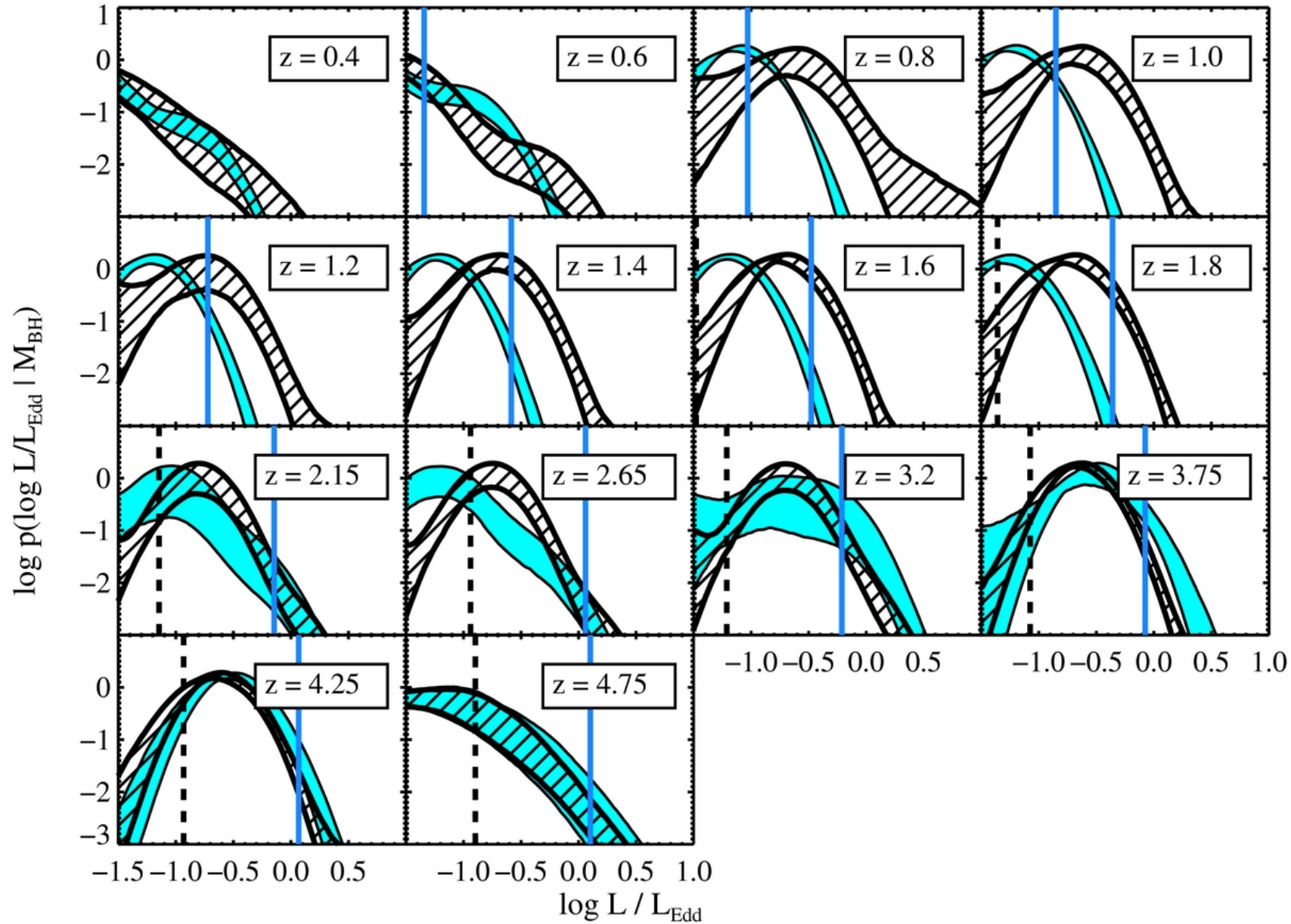
Figure 12. from The Demographics of Broad-line Quasars in the Mass-Luminosity Plane. II. Black Hole Mass and Eddington Ratio Functions Kelly & Shen 2013 ApJ 764 45 doi:10.1088/0004-637X/764/1/45 https://dx.doi.org/10.1088/0004-637X/764/1/45 © 2013. The American Astronomical Society. All rights reserved.
