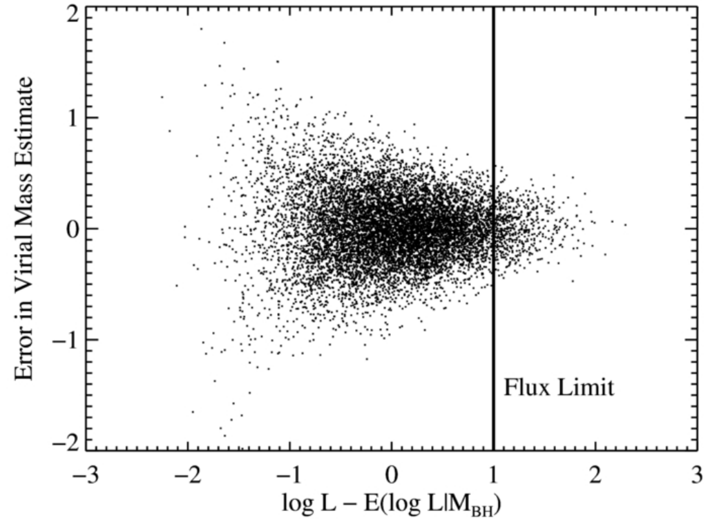
Figure 1. from The Demographics of Broad-line Quasars in the Mass-Luminosity Plane. II. Black Hole Mass and Eddington Ratio Functions Kelly & Shen 2013 ApJ 764 45 doi:10.1088/0004-637X/764/1/45 https://dx.doi.org/10.1088/0004-637X/764/1/45 © 2013. The American Astronomical Society. All rights reserved.
