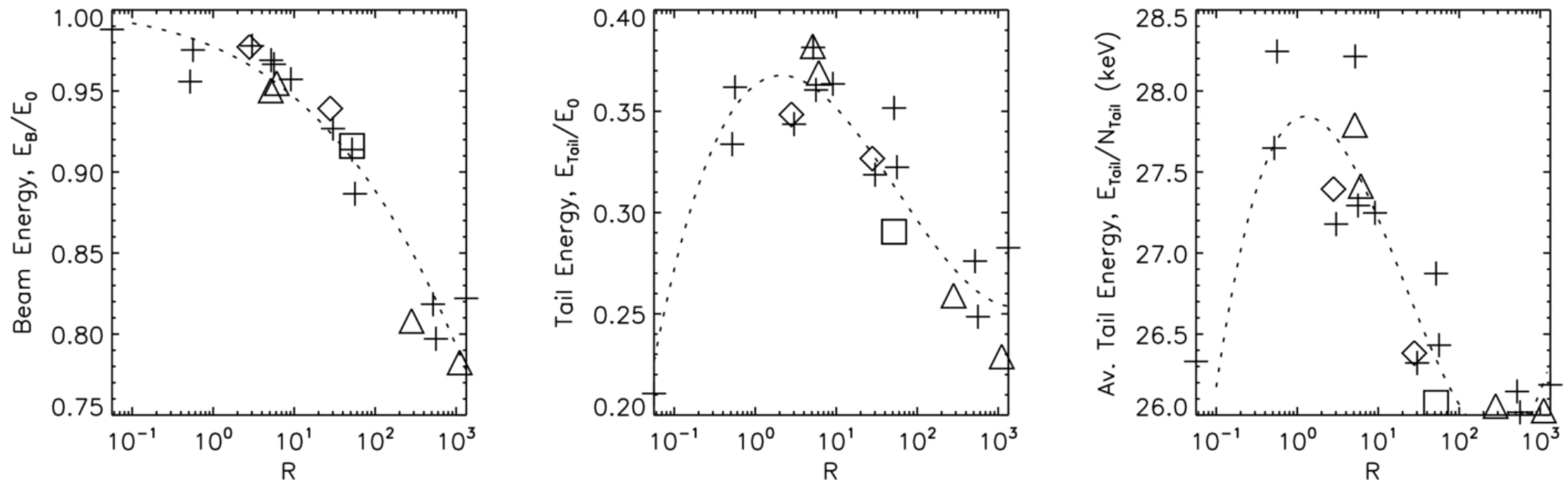
Figure 3. from Density Fluctuations and the Acceleration of Electrons by Beam-generated Langmuir Waves in the Solar Corona Ratcliffe, Bian, & Kontar 2012 ApJ 761 176 doi:10.1088/0004-637X/761/2/176 https://dx.doi.org/10.1088/0004-637X/761/2/176
