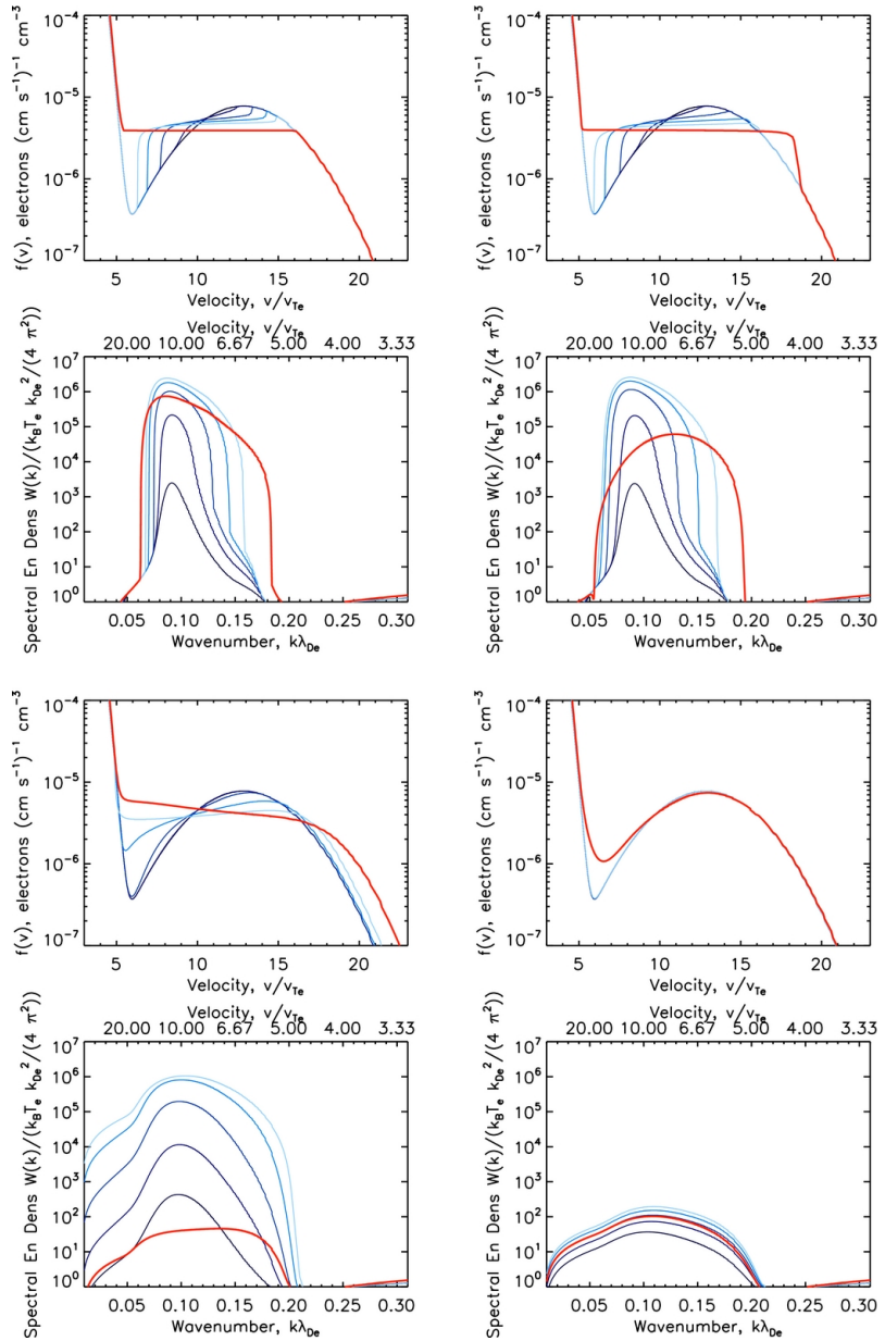
Figure 1. from Density Fluctuations and the Acceleration of Electrons by Beam-generated Langmuir Waves in the Solar Corona Ratcliffe, Bian, & Kontar 2012 ApJ 761 176 doi:10.1088/0004-637X/761/2/176 https://dx.doi.org/10.1088/0004-637X/761/2/176
