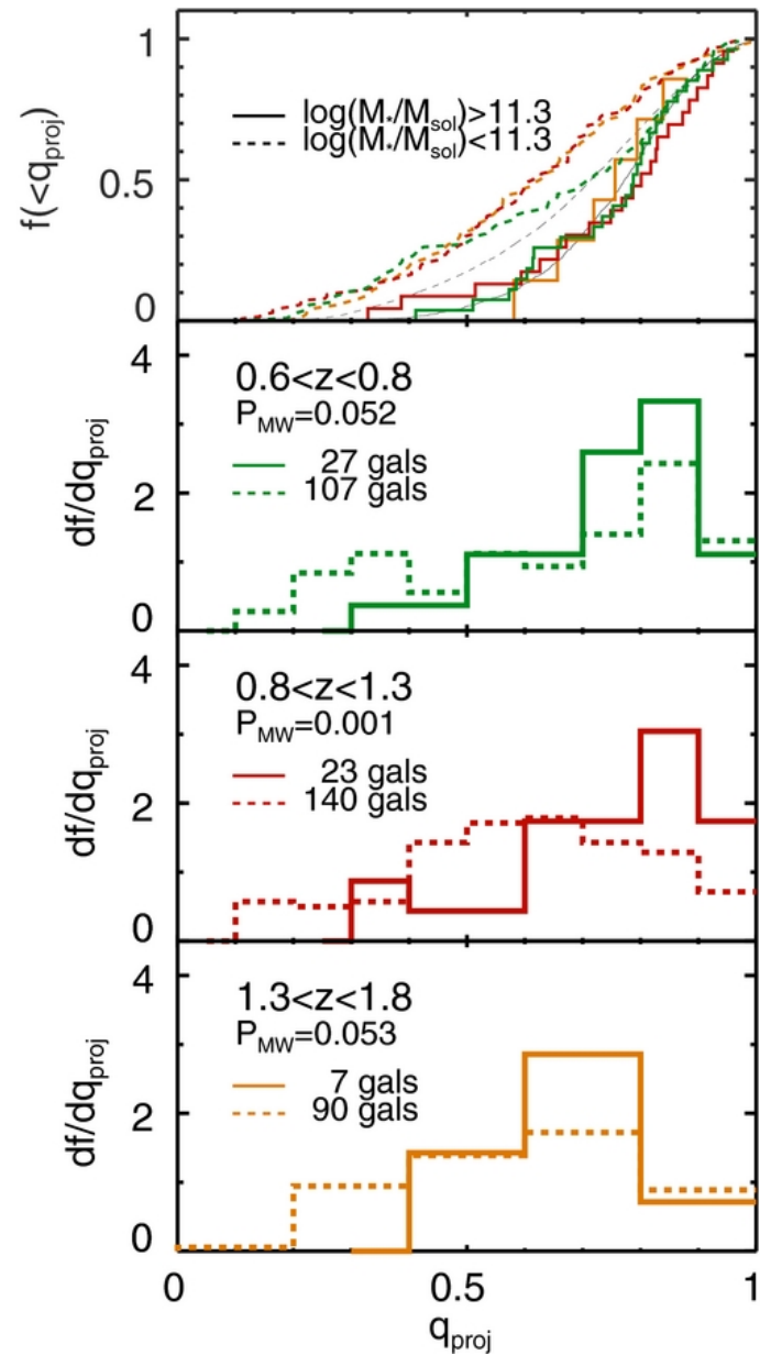
Figure 8. from Shape Evolution of Massive Early-type Galaxies: Confirmation of Increased Disk Prevalence at z > 1 Chang et al. 2013 ApJ 762 83 doi:10.1088/0004-637X/762/2/83 https://dx.doi.org/10.1088/0004-637X/762/2/83 © 2013. The American Astronomical Society. All rights reserved.
