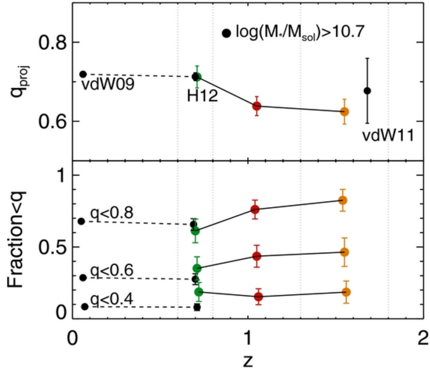
Figure 10. from Shape Evolution of Massive Early-type Galaxies: Confirmation of Increased Disk Prevalence at z > 1 Chang et al. 2013 ApJ 762 83 doi:10.1088/0004-637X/762/2/83 https://dx.doi.org/10.1088/0004-637X/762/2/83 © 2013. The American Astronomical Society. All rights reserved.
