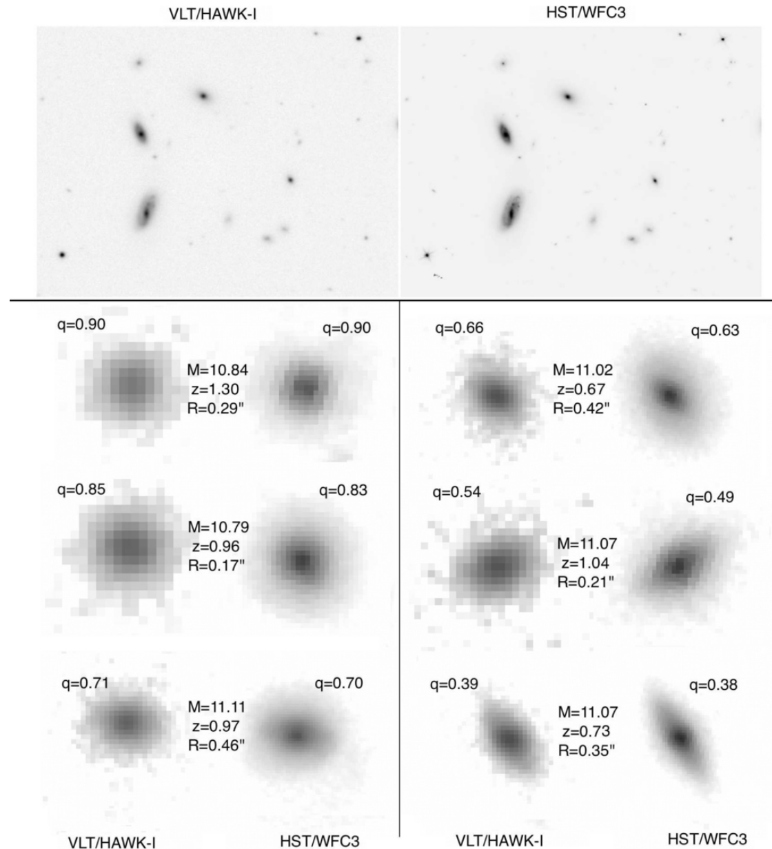
Figure 1. from Shape Evolution of Massive Early-type Galaxies: Confirmation of Increased Disk Prevalence at z > 1 Chang et al. 2013 ApJ 762 83 doi:10.1088/0004-637X/762/2/83 https://dx.doi.org/10.1088/0004-637X/762/2/83 © 2013. The American Astronomical Society. All rights reserved.
