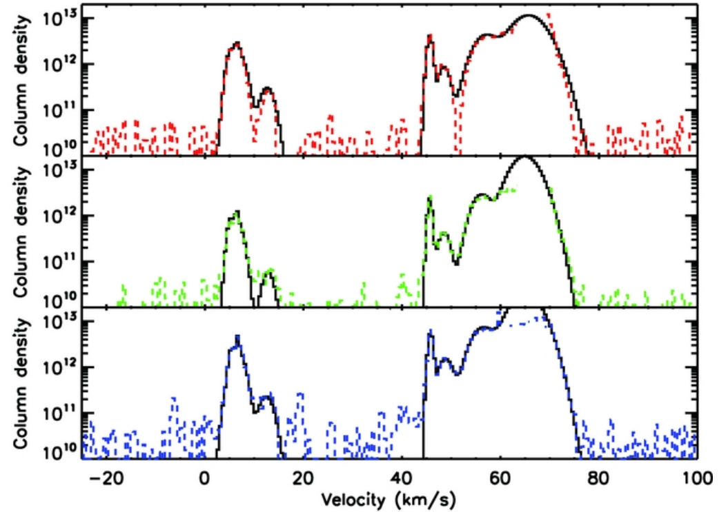
(b) Column density in the lower level
