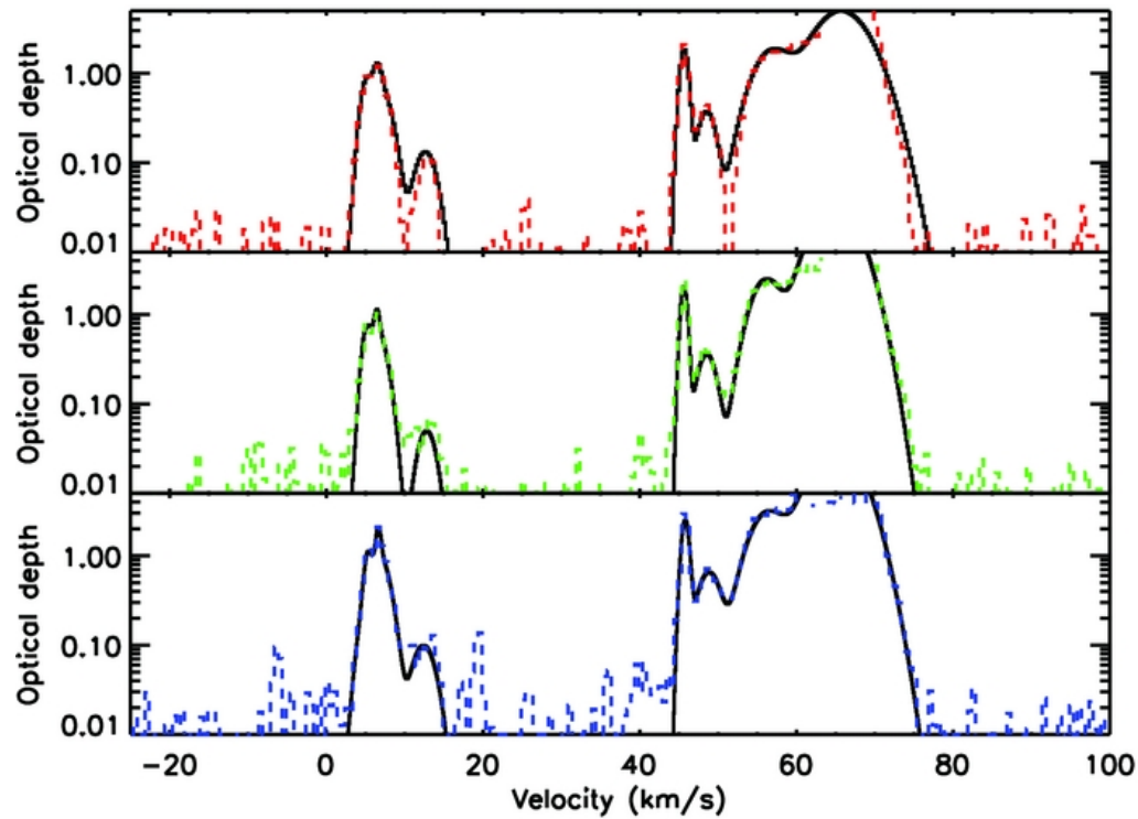
(a) Optical depth
