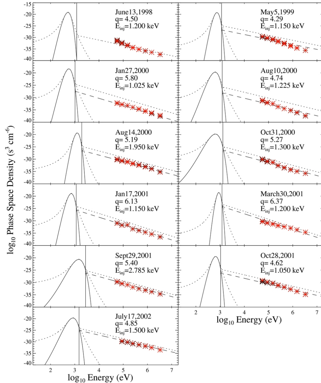
Figure 8. from Erratum: “Particle Acceleration at Quasi-parallel Shock Waves: Theory and Observations at 1 AU” (2012, ApJ, 757, 97) Erratum: 2012, ApJ, 757, 97 2012 ApJ 761 81 doi:10.1088/0004-637X/761/1/81 https://dx.doi.org/10.1088/0004-637X/761/1/81
