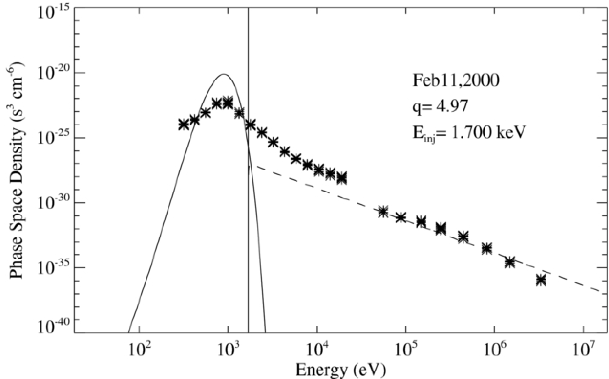
Figure 7. from Erratum: “Particle Acceleration at Quasi-parallel Shock Waves: Theory and Observations at 1 AU” (2012, ApJ, 757, 97) Erratum: 2012, ApJ, 757, 97 2012 ApJ 761 81 doi:10.1088/0004-637X/761/1/81 https://dx.doi.org/10.1088/0004-637X/761/1/81 © 2012. The American Astronomical Society. All rights reserved.
