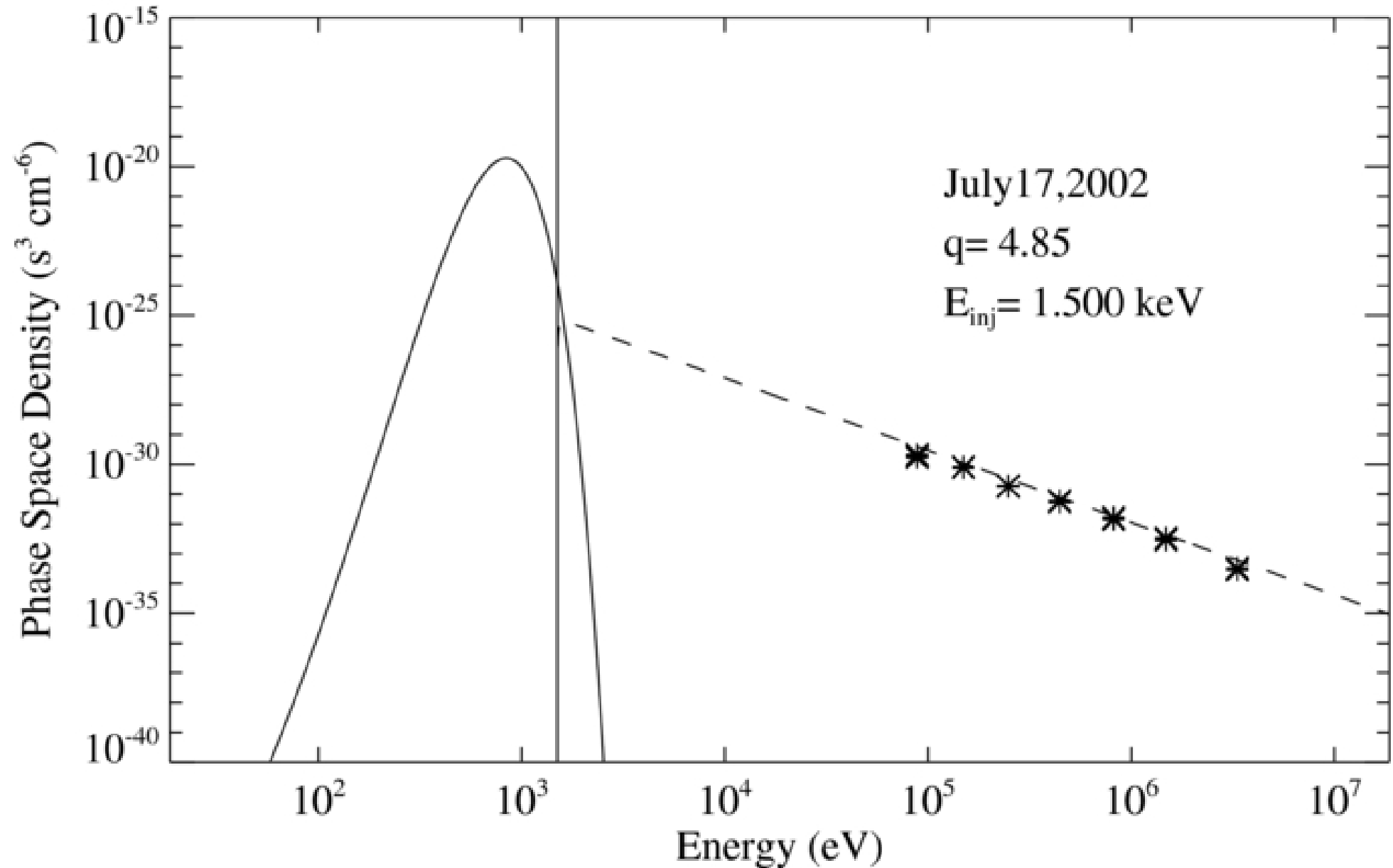
Figure 2. from Erratum: "Particle Acceleration at Quasi-parallel Shock Waves: Theory and Observations at 1 AU" (2012, ApJ, 757, 97) Erratum: 2012, ApJ, 757, 97 2012 ApJ 761 81 doi:10.1088/0004-637X/761/1/81 https://dx.doi.org/10.1088/0004-637X/761/1/81 © 2012. The American Astronomical Society. All rights reserved.
