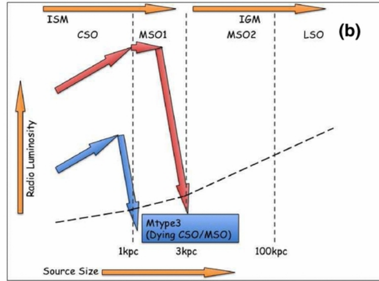
Figure 2. from The Dynamic Evolution of Young Extragalactic Radio Sources An & Baan 2012 ApJ 760 77 doi:10.1088/0004-637X/760/1/77 https://dx.doi.org/10.1088/0004-637X/760/1/77 © 2012. The American Astronomical Society. All rights reserved.
