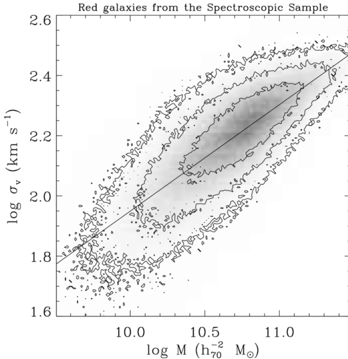
Figure 9. from Galaxy Growth by Merging in the Nearby Universe Jiang, Hogg, & Blanton 2012 ApJ 759 140 doi:10.1088/0004-637X/759/2/140 https://dx.doi.org/10.1088/0004-637X/759/2/140 © 2012. The American Astronomical Society. All rights reserved.
