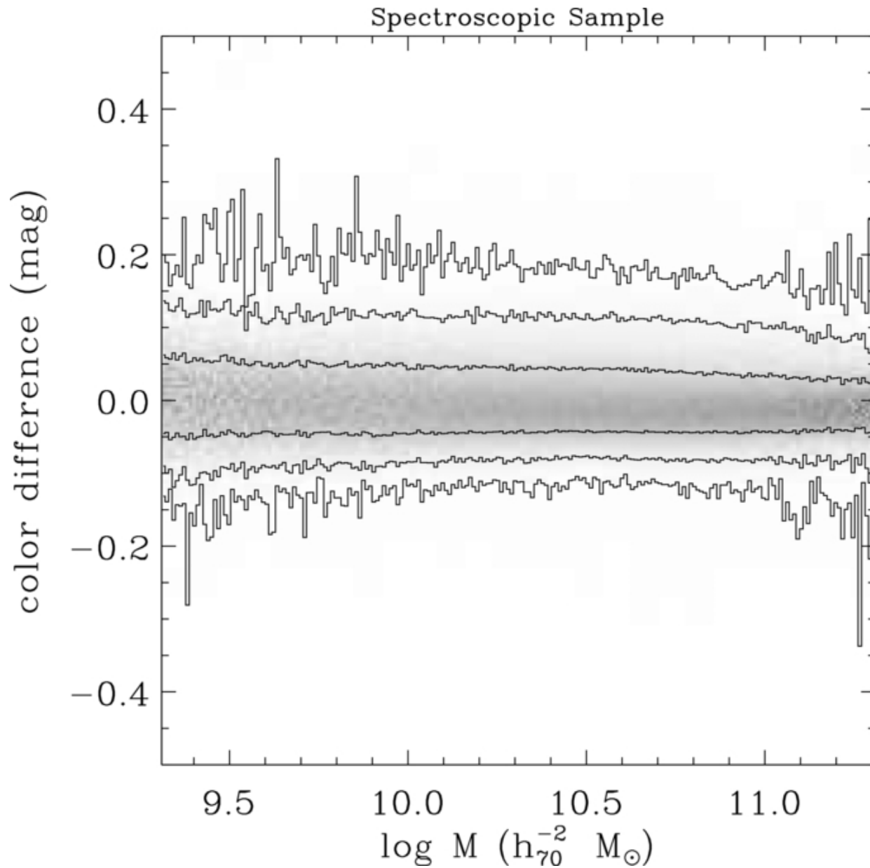
Figure 8. from Galaxy Growth by Merging in the Nearby Universe Jiang, Hogg, & Blanton 2012 ApJ 759 140 doi:10.1088/0004-637X/759/2/140 https://dx.doi.org/10.1088/0004-637X/759/2/140 © 2012. The American Astronomical Society. All rights reserved.
