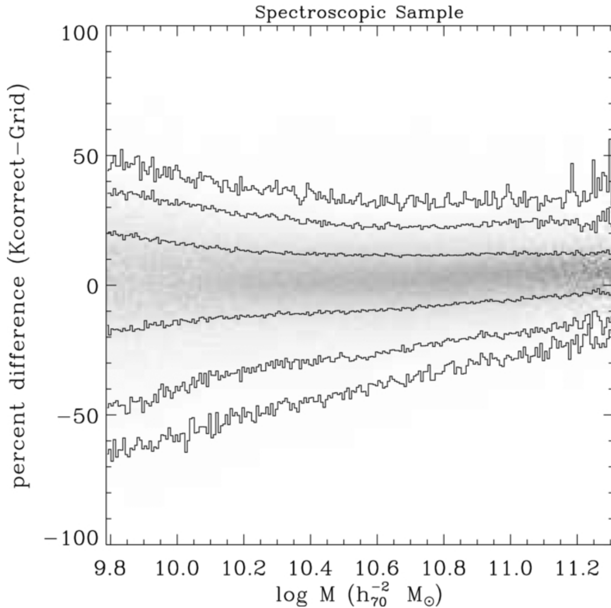
Figure 7. from Galaxy Growth by Merging in the Nearby Universe Jiang, Hogg, & Blanton 2012 ApJ 759 140 doi:10.1088/0004-637X/759/2/140 https://dx.doi.org/10.1088/0004-637X/759/2/140 © 2012. The American Astronomical Society. All rights reserved.
