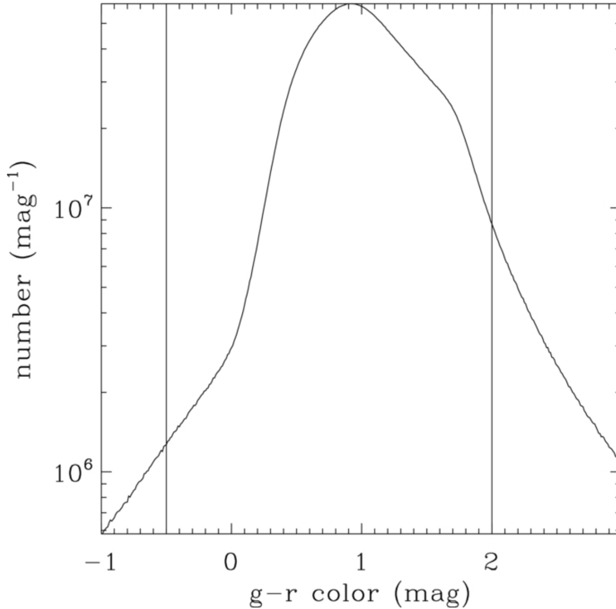
Figure 6. from Galaxy Growth by Merging in the Nearby Universe Jiang, Hogg, & Blanton 2012 ApJ 759 140 doi:10.1088/0004-637X/759/2/140 https://dx.doi.org/10.1088/0004-637X/759/2/140 © 2012. The American Astronomical Society. All rights reserved.
