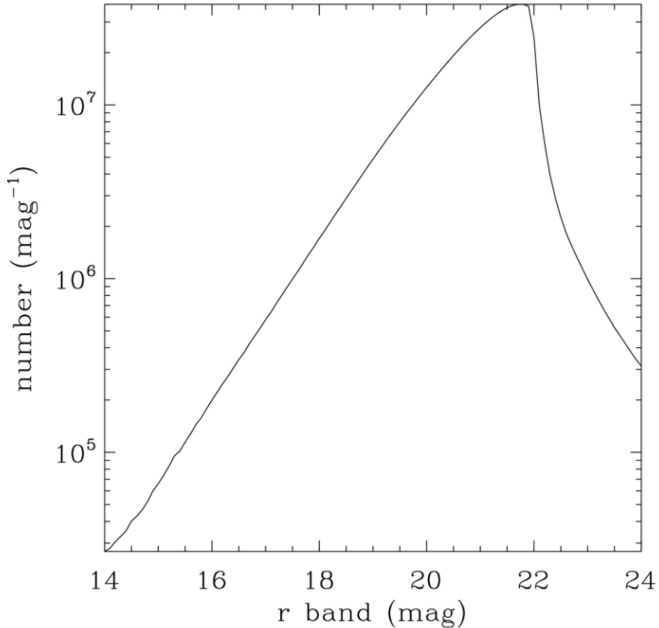
Figure 5. from Galaxy Growth by Merging in the Nearby Universe Jiang, Hogg, & Blanton 2012 ApJ 759 140 doi:10.1088/0004-637X/759/2/140 https://dx.doi.org/10.1088/0004-637X/759/2/140 © 2012. The American Astronomical Society. All rights reserved.
