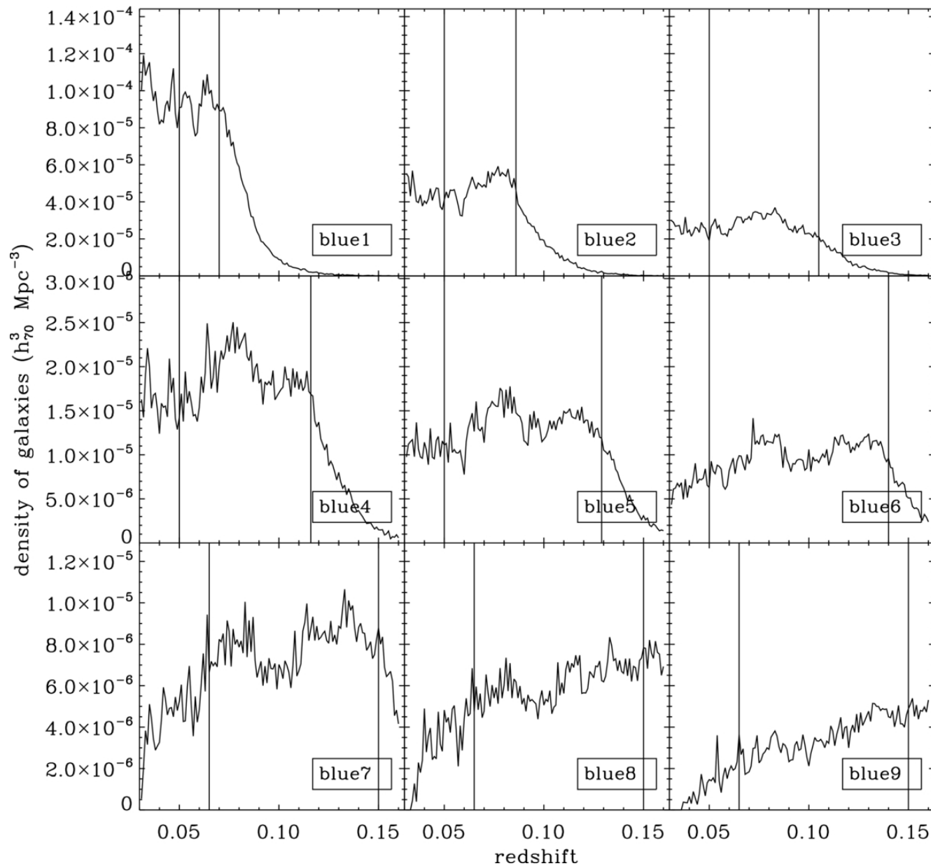
Figure 4. from Galaxy Growth by Merging in the Nearby Universe Jiang, Hogg, & Blanton 2012 ApJ 759 140 doi:10.1088/0004-637X/759/2/140 https://dx.doi.org/10.1088/0004-637X/759/2/140 © 2012. The American Astronomical Society. All rights reserved.
