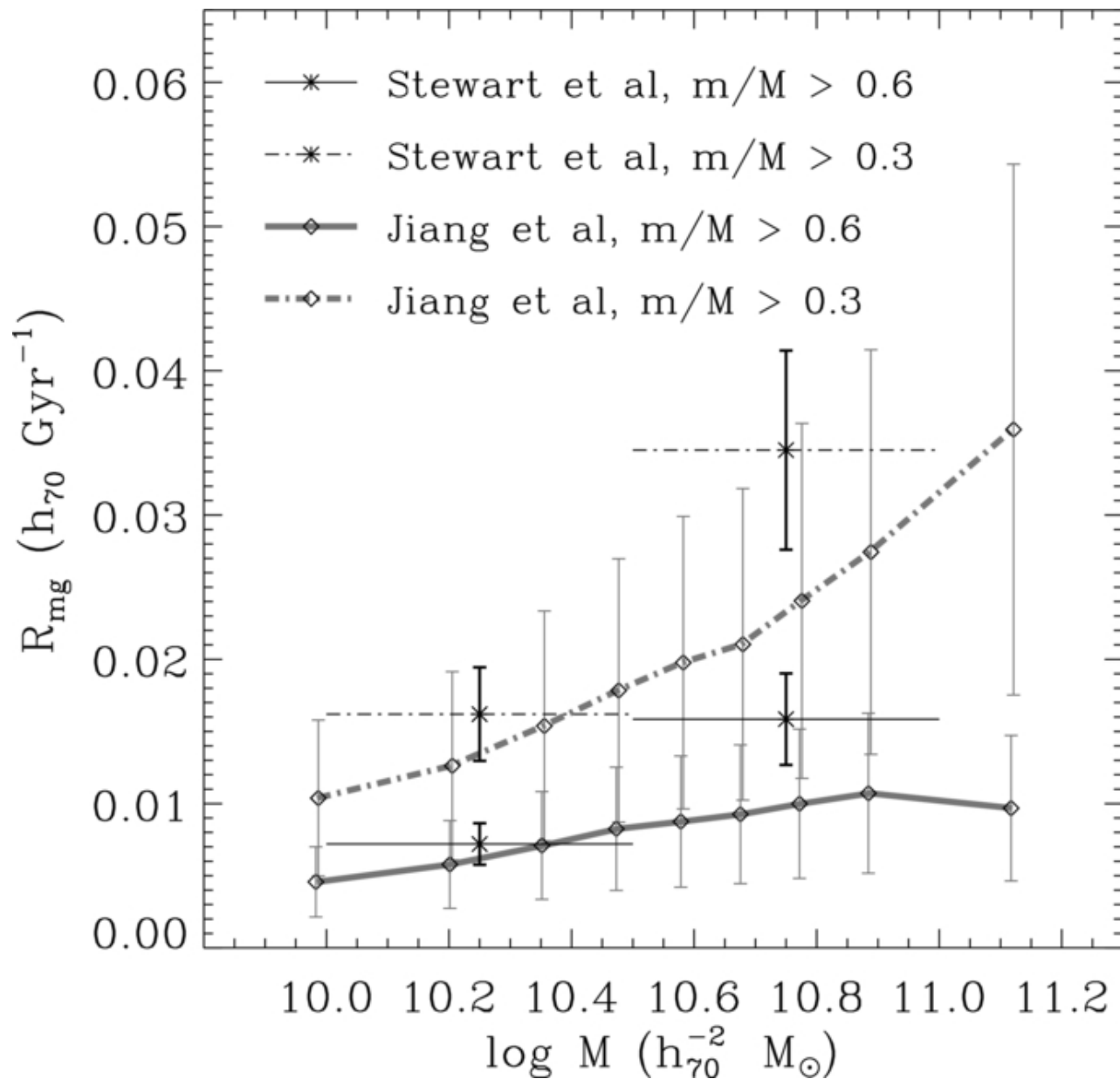
Figure 26. from Galaxy Growth by Merging in the Nearby Universe Jiang, Hogg, & Blanton 2012 ApJ 759 140 doi:10.1088/0004-637X/759/2/140 https://dx.doi.org/10.1088/0004-637X/759/2/140 © 2012. The American Astronomical Society. All rights reserved.
