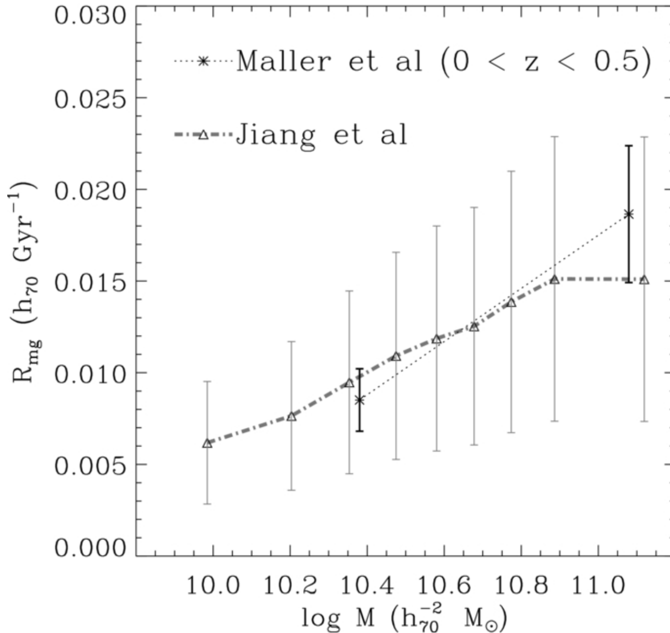
Figure 25. from Galaxy Growth by Merging in the Nearby Universe Jiang, Hogg, & Blanton 2012 ApJ 759 140 doi:10.1088/0004-637X/759/2/140 https://dx.doi.org/10.1088/0004-637X/759/2/140 © 2012. The American Astronomical Society. All rights reserved.
