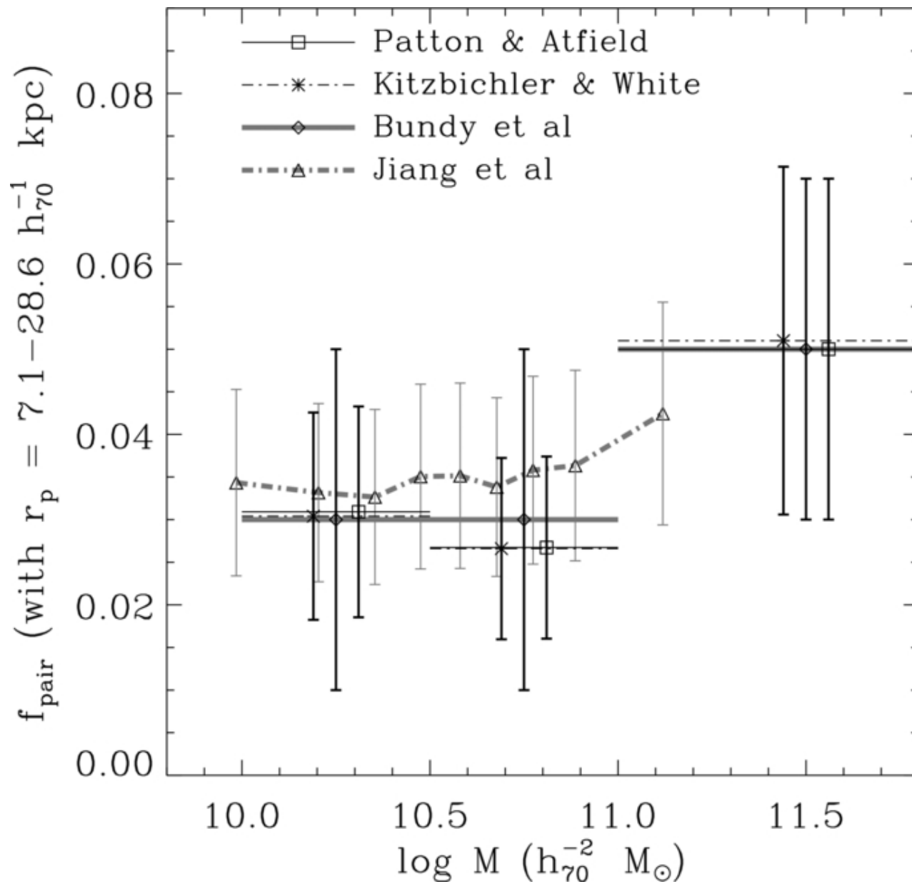
Figure 24. from Galaxy Growth by Merging in the Nearby Universe Jiang, Hogg, & Blanton 2012 ApJ 759 140 doi:10.1088/0004-637X/759/2/140 https://dx.doi.org/10.1088/0004-637X/759/2/140 © 2012. The American Astronomical Society. All rights reserved.
