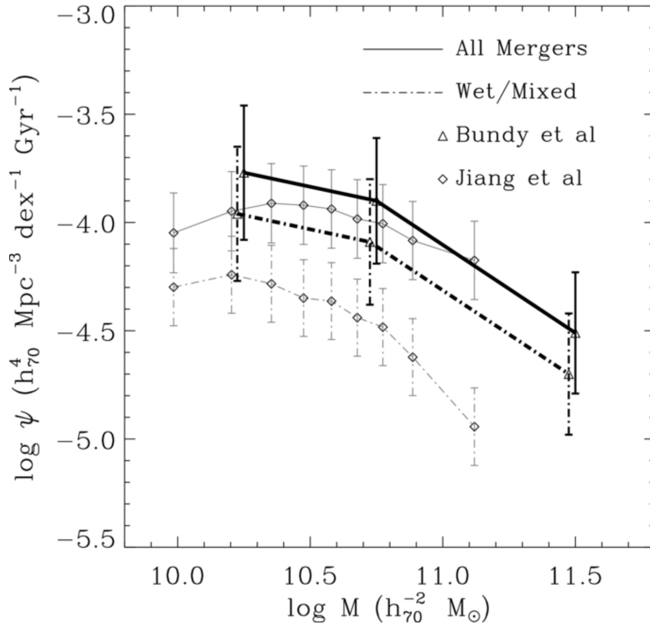
Figure 23. from Galaxy Growth by Merging in the Nearby Universe Jiang, Hogg, & Blanton 2012 ApJ 759 140 doi:10.1088/0004-637X/759/2/140 https://dx.doi.org/10.1088/0004-637X/759/2/140 © 2012. The American Astronomical Society. All rights reserved.
