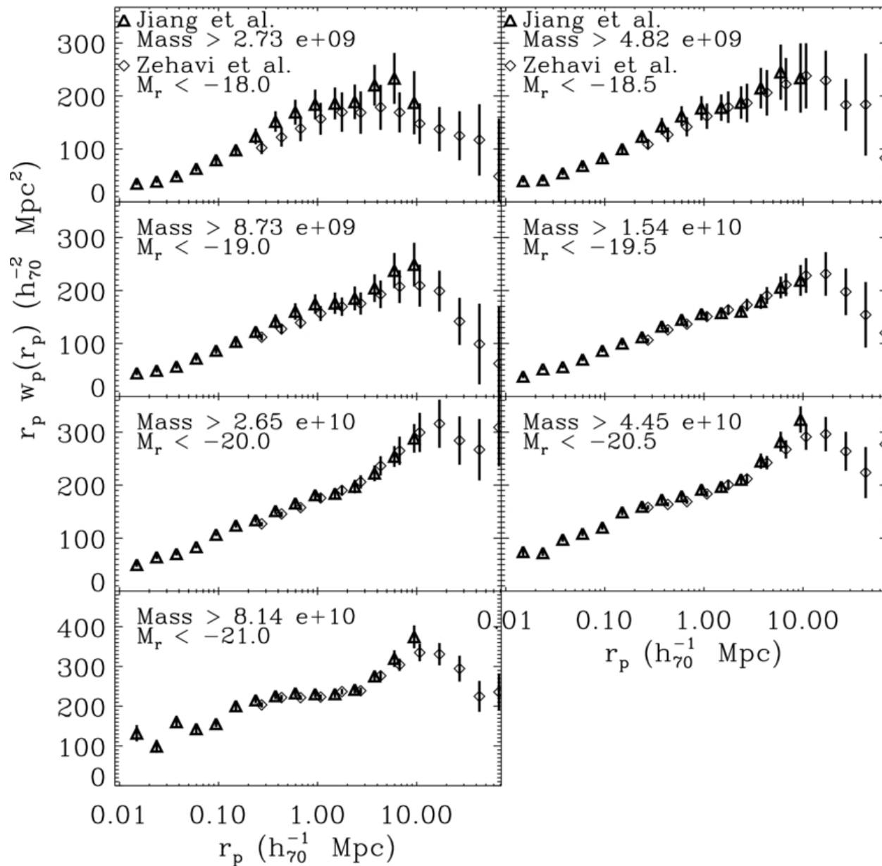
Figure 20. from Galaxy Growth by Merging in the Nearby Universe Jiang, Hogg, & Blanton 2012 ApJ 759 140 doi:10.1088/0004-637X/759/2/140 https://dx.doi.org/10.1088/0004-637X/759/2/140 © 2012. The American Astronomical Society. All rights reserved.
