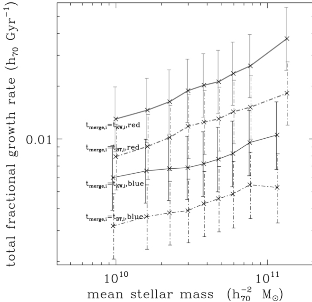
Figure 19. from Galaxy Growth by Merging in the Nearby Universe Jiang, Hogg, & Blanton 2012 ApJ 759 140 doi:10.1088/0004-637X/759/2/140 https://dx.doi.org/10.1088/0004-637X/759/2/140 © 2012. The American Astronomical Society. All rights reserved.
