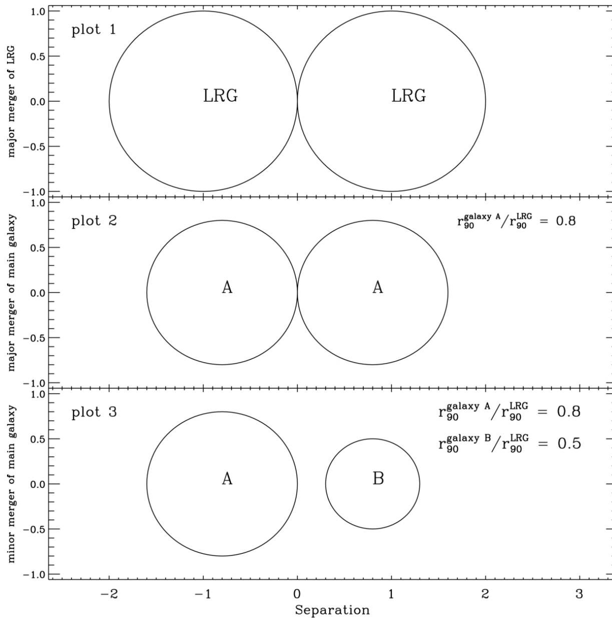
Figure 16. from Galaxy Growth by Merging in the Nearby Universe Jiang, Hogg, & Blanton 2012 ApJ 759 140 doi:10.1088/0004-637X/759/2/140 https://dx.doi.org/10.1088/0004-637X/759/2/140 © 2012. The American Astronomical Society. All rights reserved.
