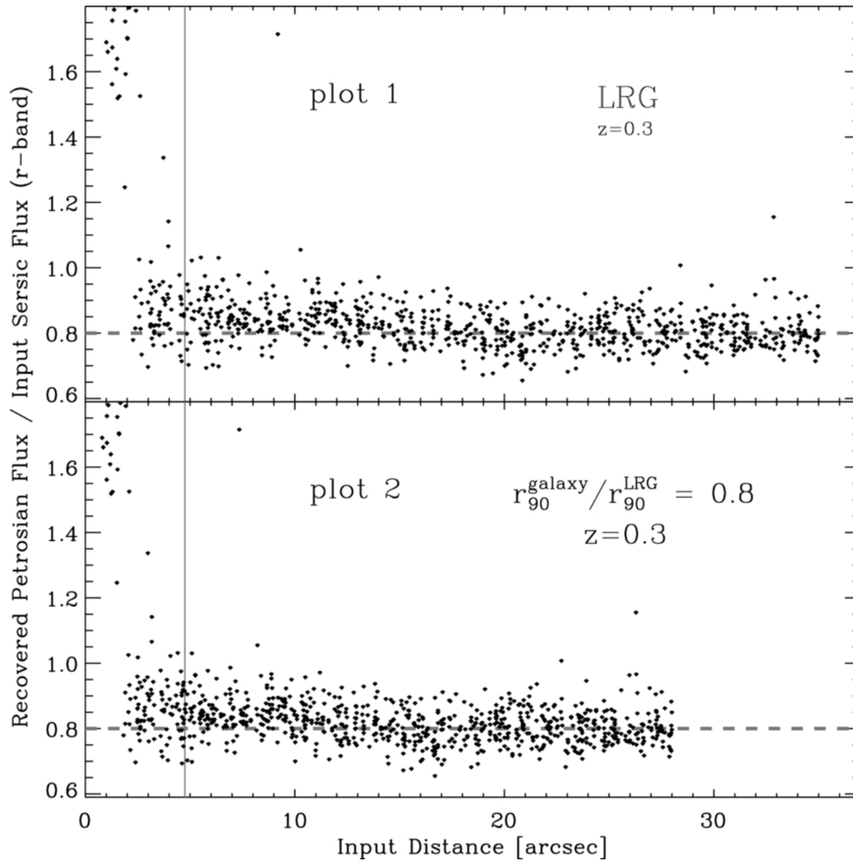
Figure 14. from Galaxy Growth by Merging in the Nearby Universe Jiang, Hogg, & Blanton 2012 ApJ 759 140 doi:10.1088/0004-637X/759/2/140 https://dx.doi.org/10.1088/0004-637X/759/2/140 © 2012. The American Astronomical Society. All rights reserved.
