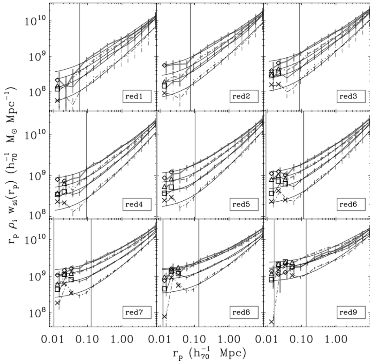
Figure 11. from Galaxy Growth by Merging in the Nearby Universe Jiang, Hogg, & Blanton 2012 ApJ 759 140 doi:10.1088/0004-637X/759/2/140 https://dx.doi.org/10.1088/0004-637X/759/2/140 © 2012. The American Astronomical Society. All rights reserved.
