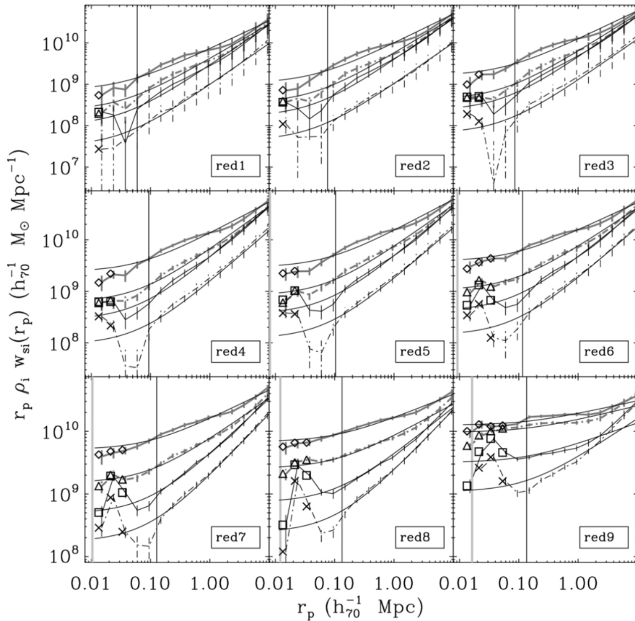
Figure 10. from Galaxy Growth by Merging in the Nearby Universe Jiang, Hogg, & Blanton 2012 ApJ 759 140 doi:10.1088/0004-637X/759/2/140 https://dx.doi.org/10.1088/0004-637X/759/2/140 © 2012. The American Astronomical Society. All rights reserved.
