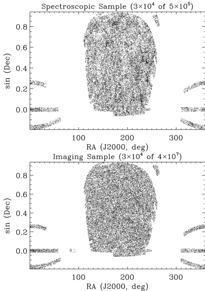
Figure 1. from Galaxy Growth by Merging in the Nearby Universe Jiang, Hogg, & Blanton 2012 ApJ 759 140 doi:10.1088/0004-637X/759/2/140 https://dx.doi.org/10.1088/0004-637X/759/2/140 © 2012. The American Astronomical Society. All rights reserved.
