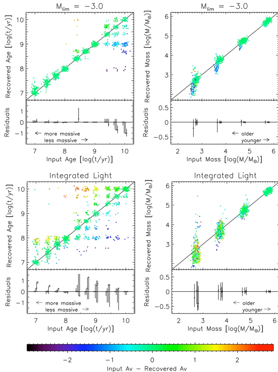
Figure 7. from The Panchromatic Hubble Andromeda Treasury. III. Measuring Ages and Masses of Partially Resolved Stellar Clusters Beerman et al. 2012 ApJ 760 104 doi:10.1088/0004-637X/760/2/104 https://dx.doi.org/10.1088/0004-637X/760/2/104
