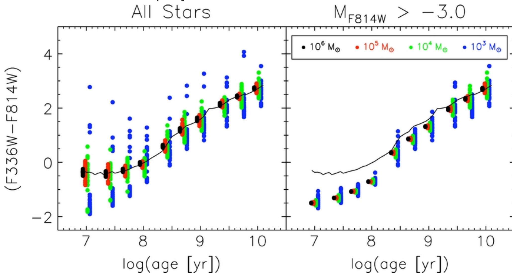
Figure 5. from The Panchromatic Hubble Andromeda Treasury. III. Measuring Ages and Masses of Partially Resolved Stellar Clusters Beerman et al. 2012 ApJ 760 104 doi:10.1088/0004-637X/760/2/104 https://dx.doi.org/10.1088/0004-637X/760/2/104 © 2012. The American Astronomical Society. All rights reserved.
