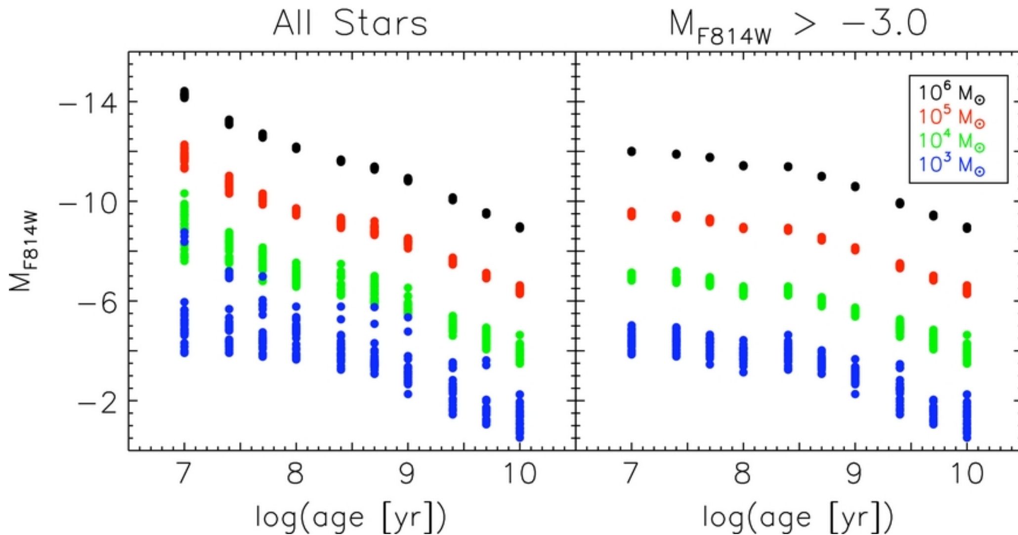
Figure 4. from The Panchromatic Hubble Andromeda Treasury. III. Measuring Ages and Masses of Partially Resolved Stellar Clusters Beerman et al. 2012 ApJ 760 104 doi:10.1088/0004-637X/760/2/104 https://dx.doi.org/10.1088/0004-637X/760/2/104 © 2012. The American Astronomical Society. All rights reserved.
