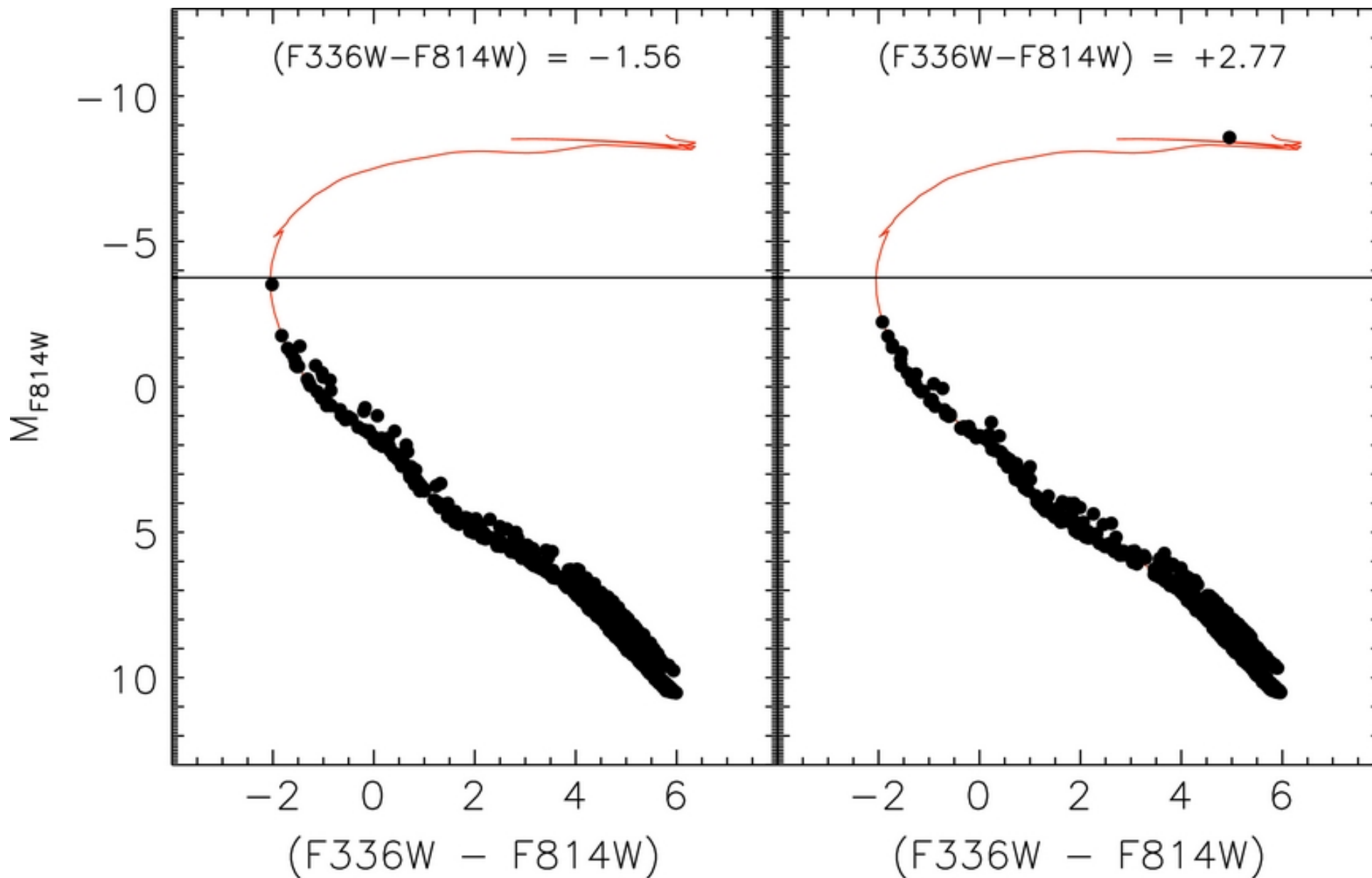
Figure 1. from The Panchromatic Hubble Andromeda Treasury. III. Measuring Ages and Masses of Partially Resolved Stellar Clusters Beerman et al. 2012 ApJ 760 104 doi:10.1088/0004-637X/760/2/104 https://dx.doi.org/10.1088/0004-637X/760/2/104 © 2012. The American Astronomical Society. All rights reserved.
