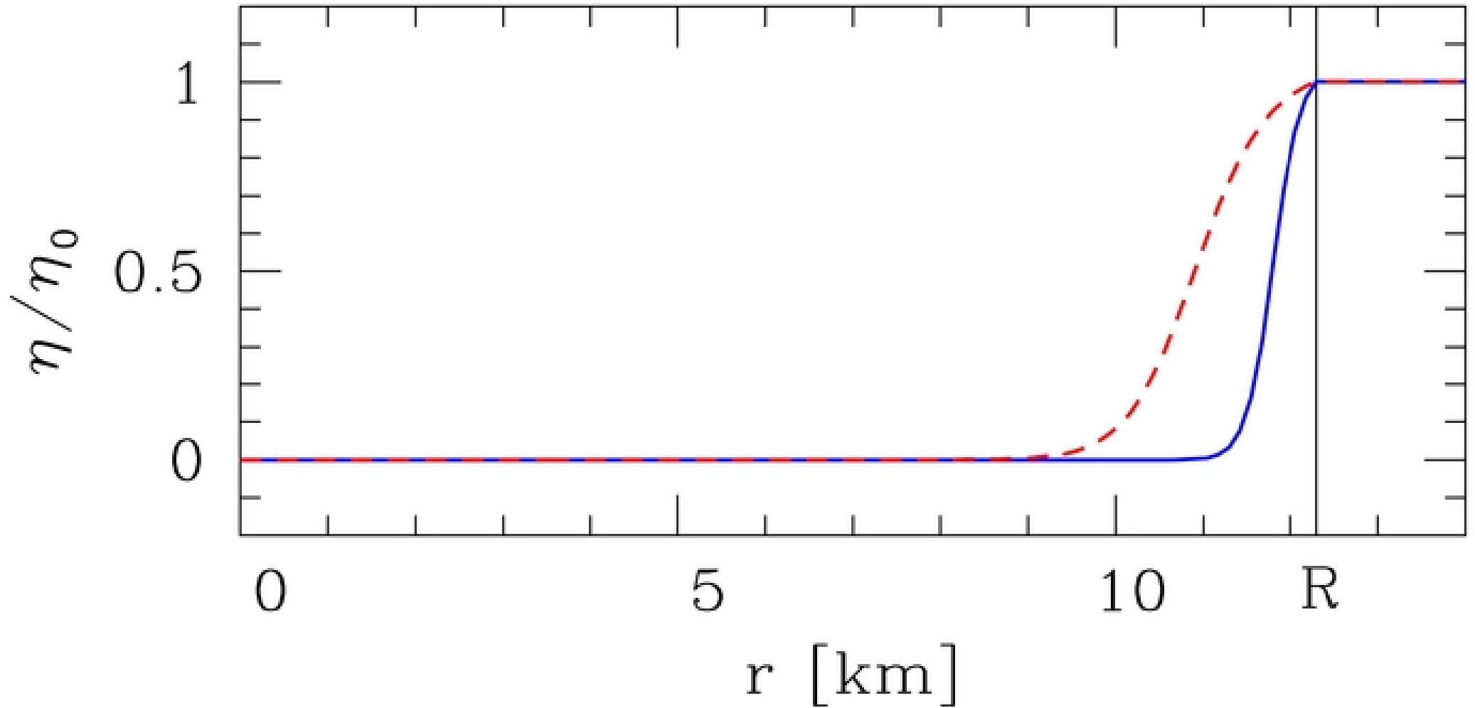
Figure 1. from Poloidal-field Instability in Magnetized Relativistic Stars Ciolfi & Rezzolla 2012 ApJ 760 1 doi:10.1088/0004-637X/760/1/1 https://dx.doi.org/10.1088/0004-637X/760/1/1 © 2012. The American Astronomical Society. All rights reserved.
